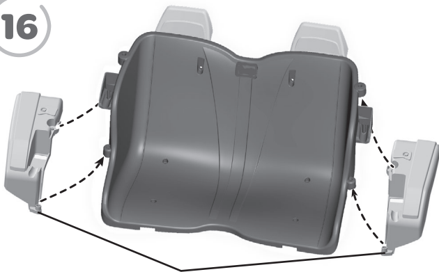
Rear Fenders Guardabarros traseros Ailes arrière
